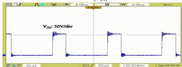
( V_{D2} )
