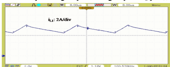
( i_{L1} )
