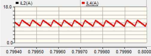
(Inductor current ripple I_{L2} = I_{L4} )
