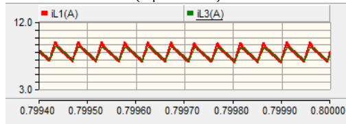
(Inductor current ripple I_{L2} = I_{L4} )
